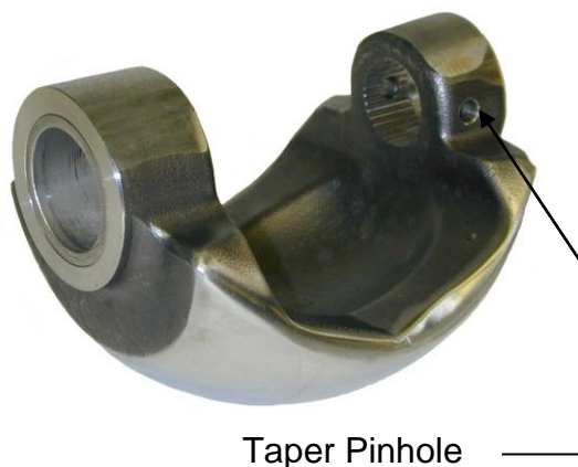
Figure 2. V-Ball showing Groove Pin Hole
