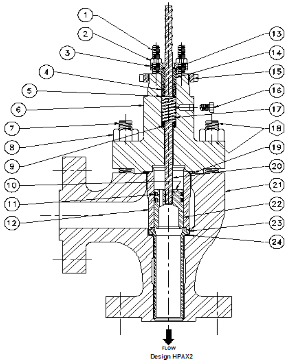
Figure 4 - 2" HPAX2 Valve
