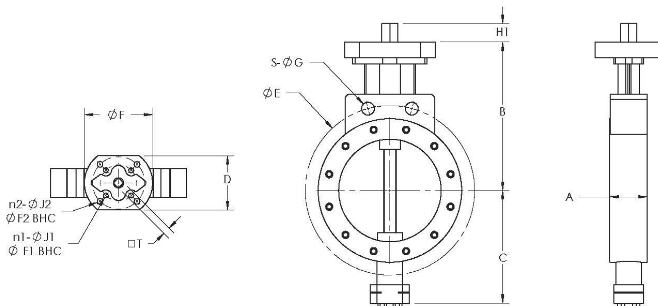
BFH200 2-12" CL 300 WAFER TYPE BUTTERFLY VALVE DIMENSIONS - Inch
